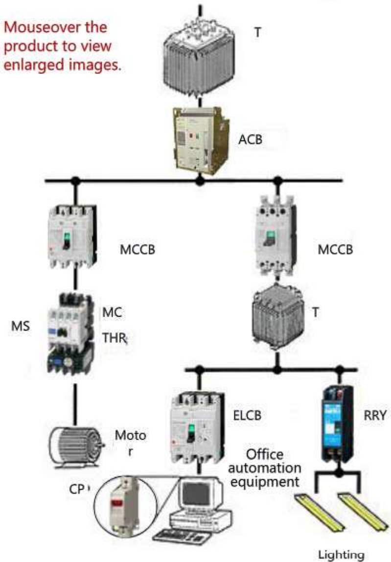
Low voltage circuits
