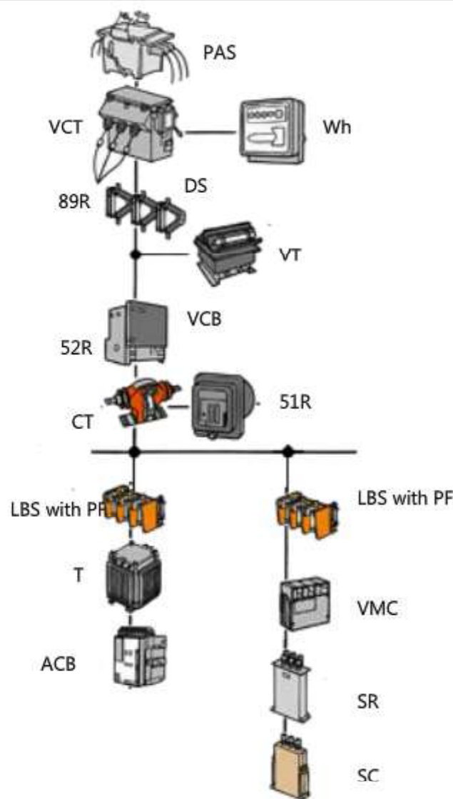
Fig.1 Cubicle type high voltage power receiving equipment
