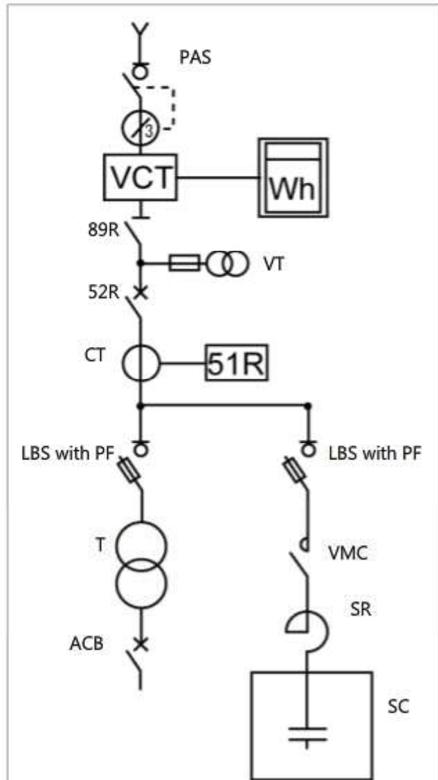
Fig.2 Skeleton (Single line connection diagram)
