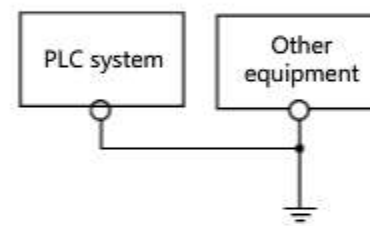
(3) Common grounding: Not allowed
