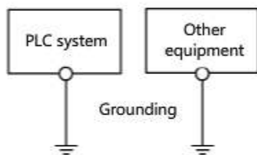
(1) Independent grounding: Recommended
