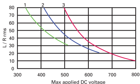
Figure I2. 1000-1250 Vac Typower Zilox maximum applied DC voltage.
