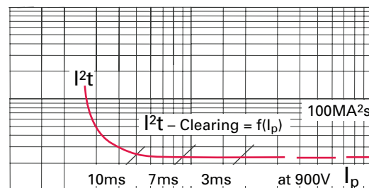
Figure C6. I^2t curve.
