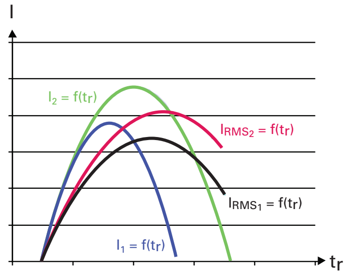
Figure C2. Overload and fault current curves.
