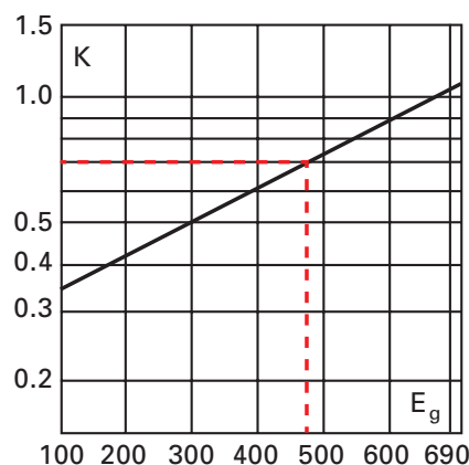
Figure L1. Reference: Bussmann series product data sheet no. 720013, total clearing I^2t at rated voltage.
