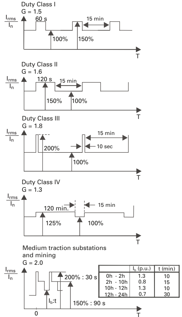
Figure E7. Cyclic loading profile examples and duty class.
