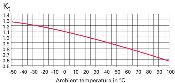
Figure E1. Ambient temperature correction factor.
