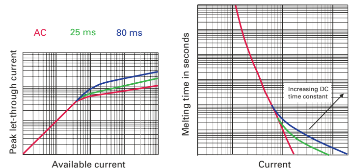
Figure H2. AC and DC operating characteristics will merge for operating times greater than 1 second.
