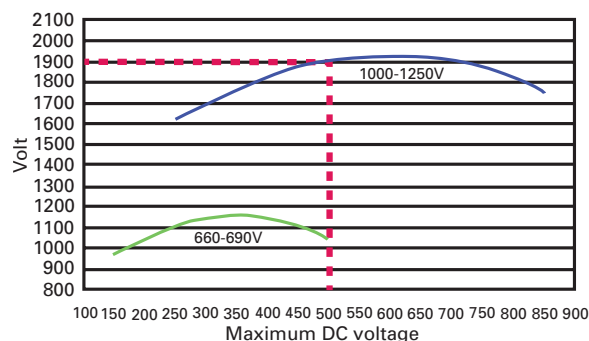
Figure I8. Worst case arc voltage.
