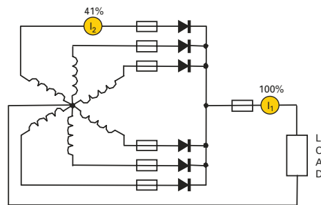
Figure F6. Six-phase, star
