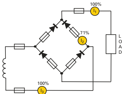
Figure F3. Single-phase, bridge
