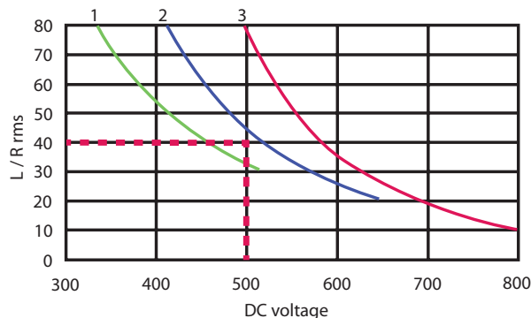
Figure I6. Maximum applied DC voltage.
