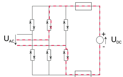
Figure L7. Regenerative drive circuit example (see Figures J1 to J6 on pages 20 to 21).
