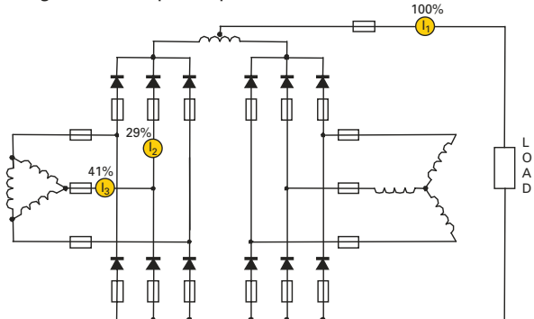
Figure F8. Six-phase parallel (with IPT)
